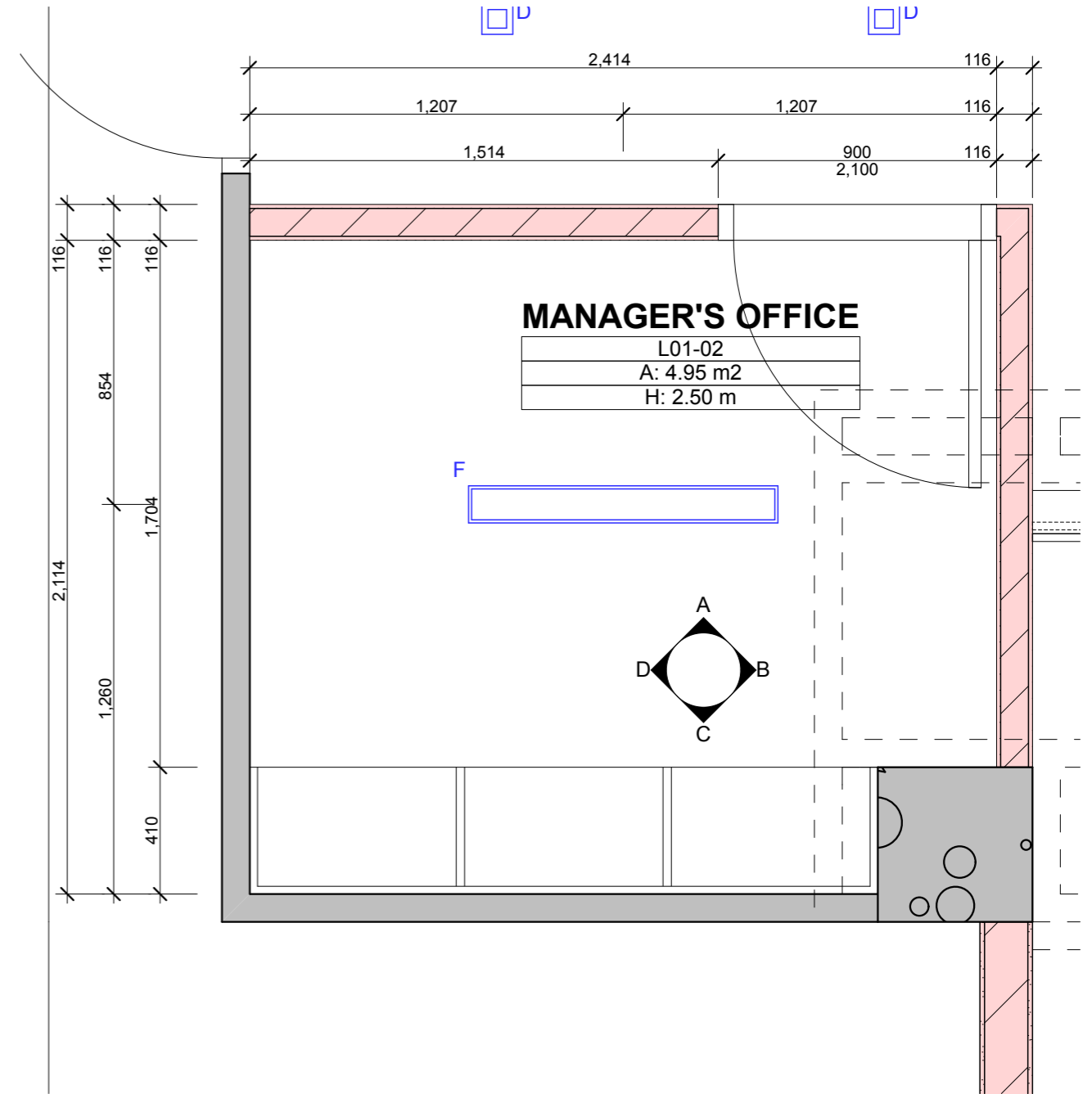
Manager's Office RCP 1:20
