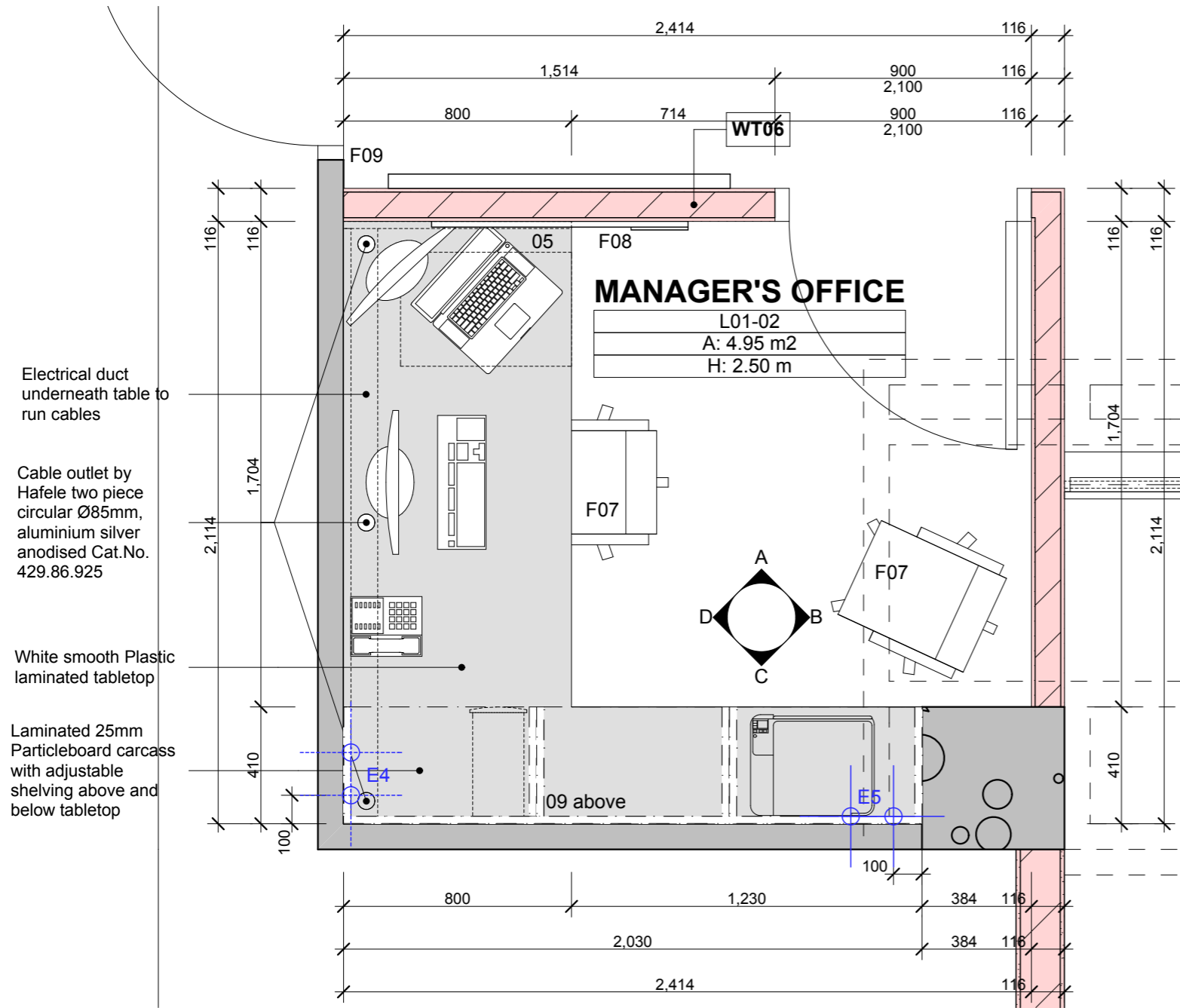
Manager's Office Plan 1:20
